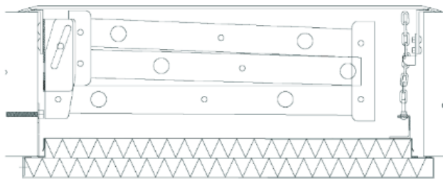
5. Cross-section of a balcony hatch with firestop
