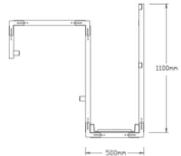
3. Cross-section of the platform
